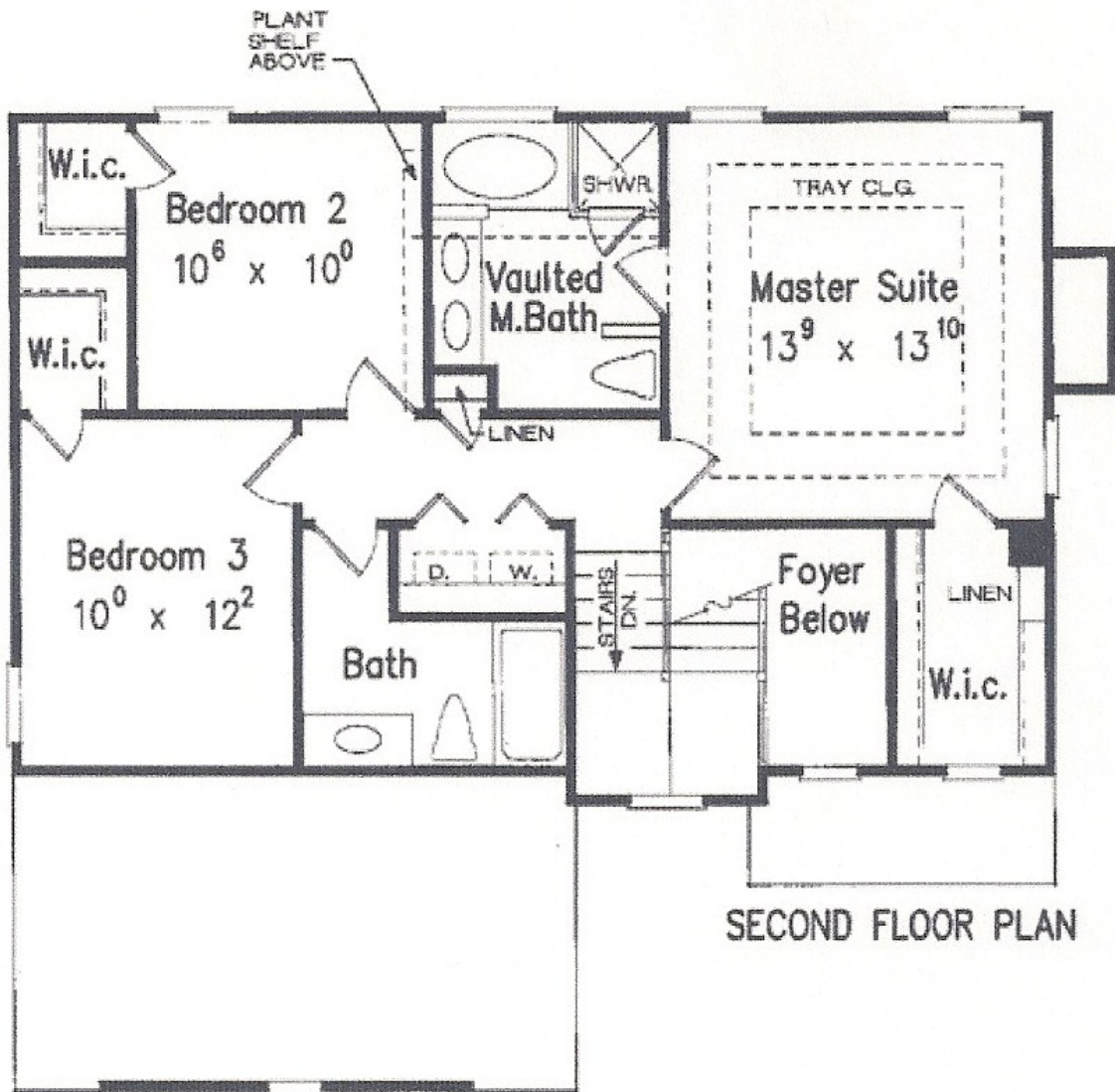
2nd Floor Plan (779 S.Q.)
