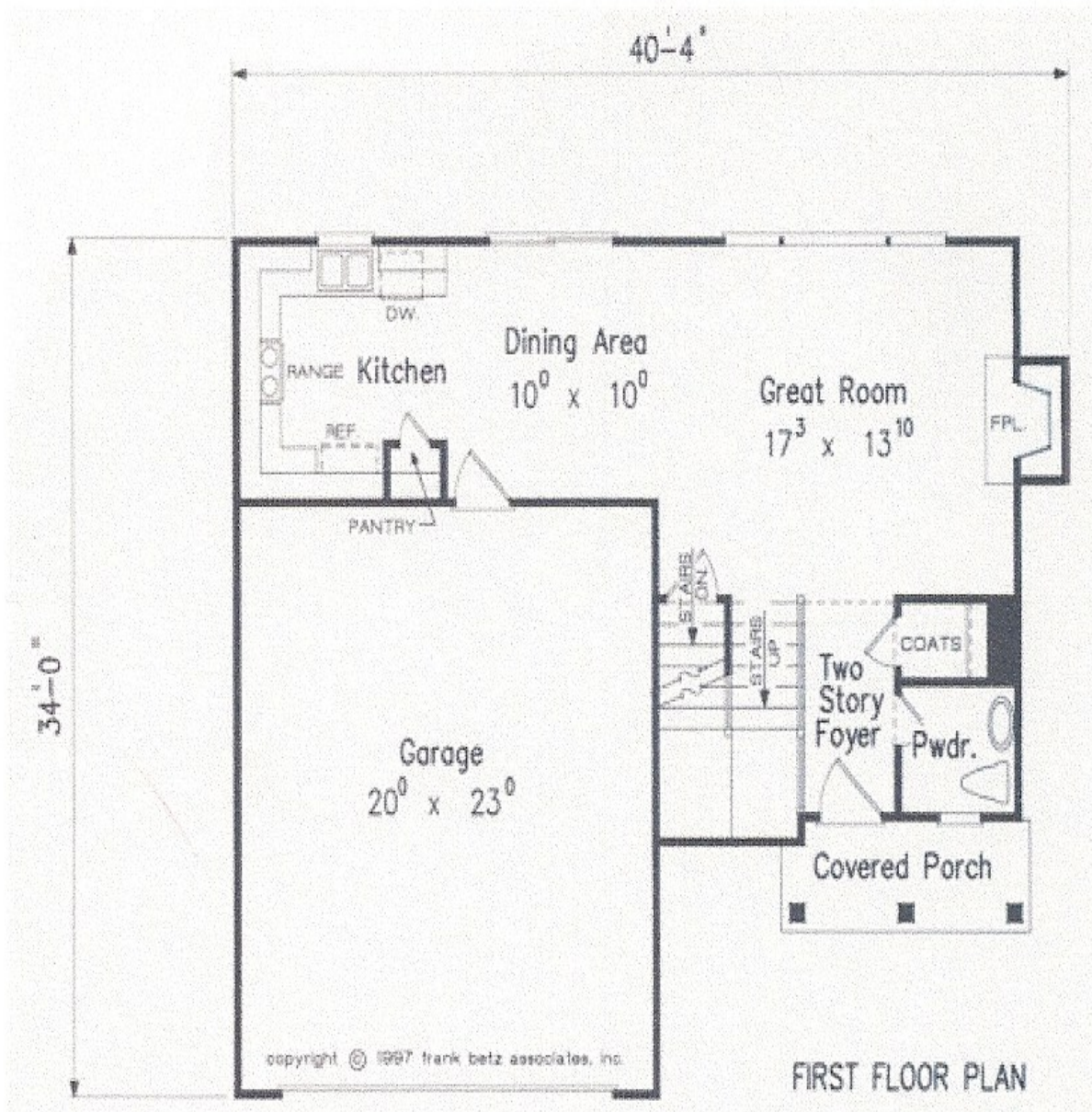
1st Floor Plan (630 S.Q.)
