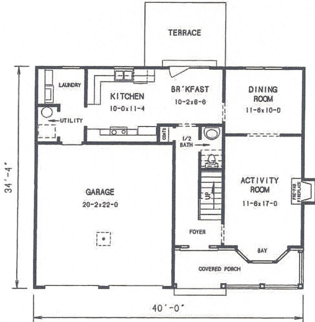
1st Floor Plan (906 S.Q.)
