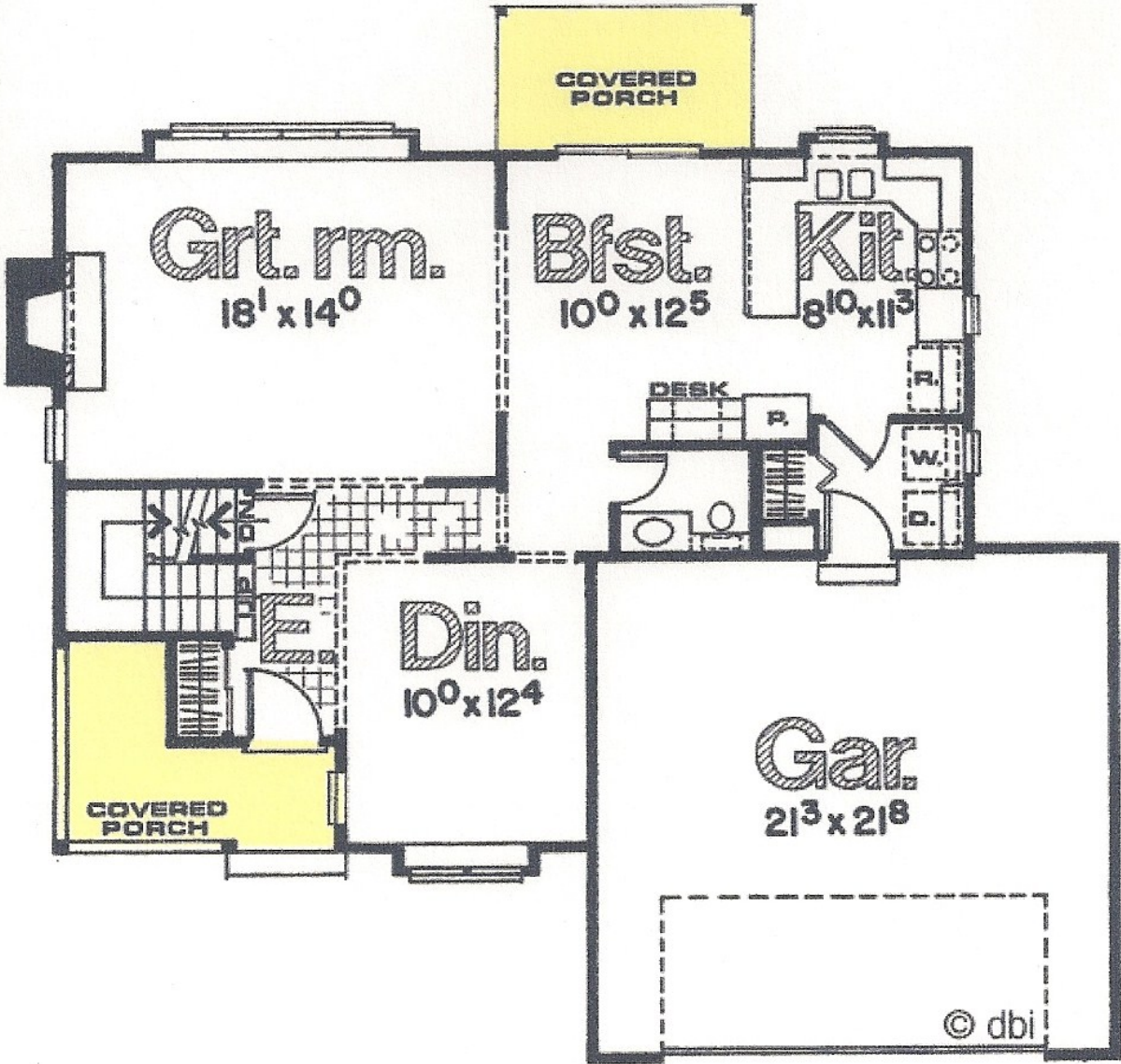
1st Floor Plan (891 S.Q.)
