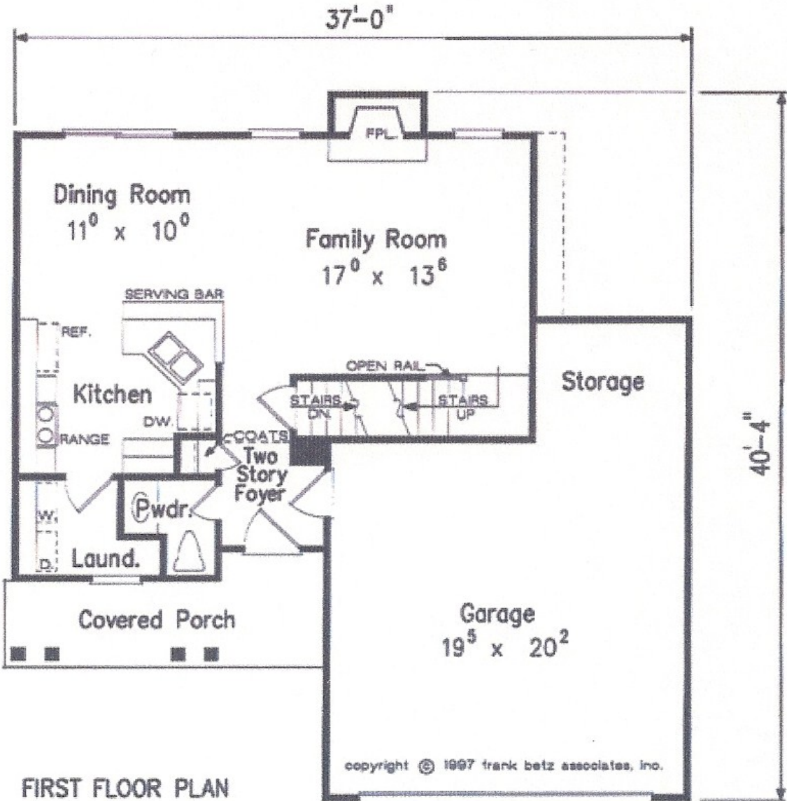
1st Floor Plan (628 S.Q.)
