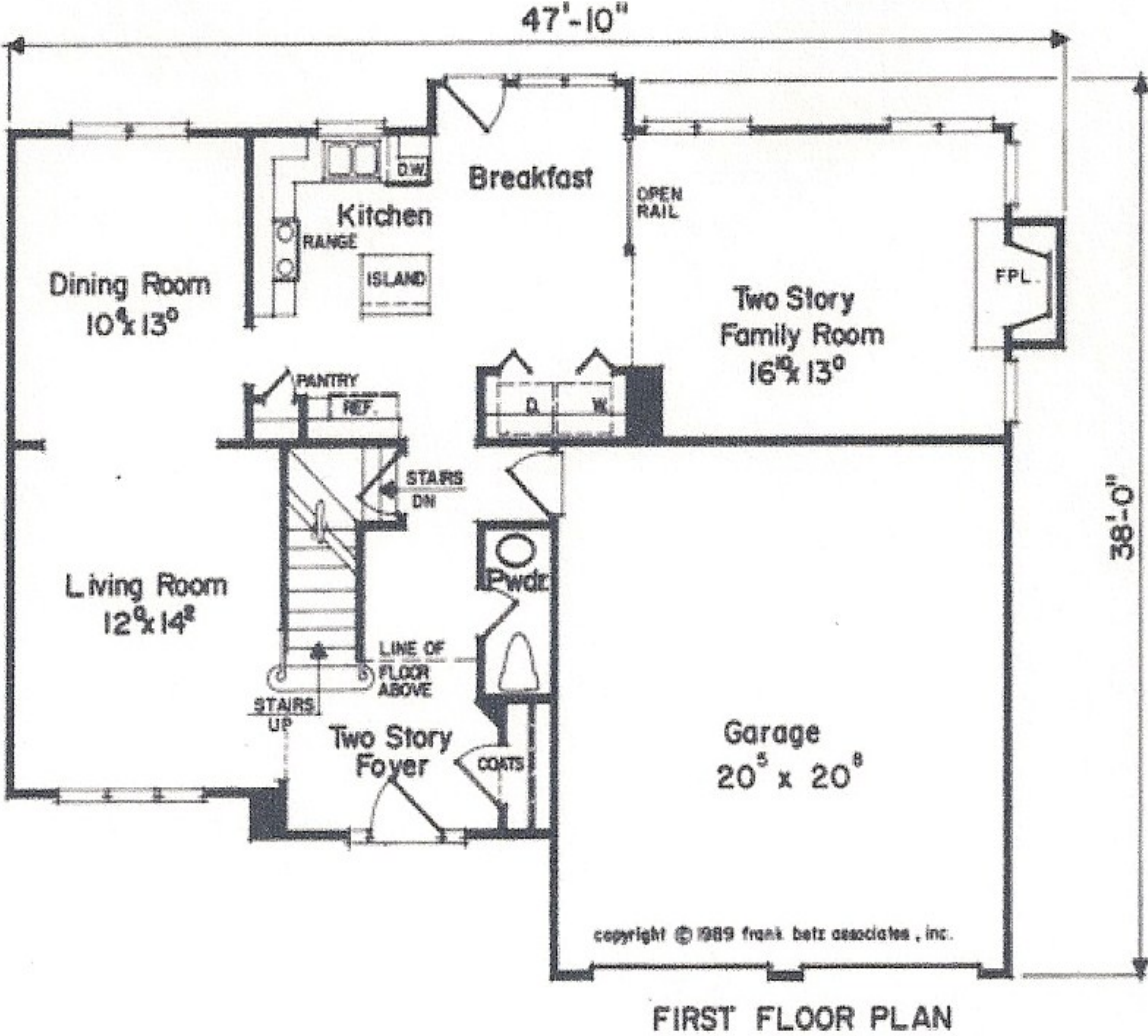
1st Floor Plan (1014 S.Q.)
